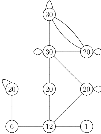
Figure 4: Representation C as a t -linkage of orbits of T = \langle a, b, c \rangle
