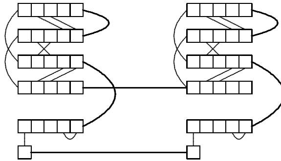
Figure 2: Representation A as a t -linkage of orbits of S = \langle b, c \rangle
