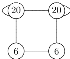
Figure 1: Representation A as a t -linkage of orbits of T = \langle a, b, c \rangle
