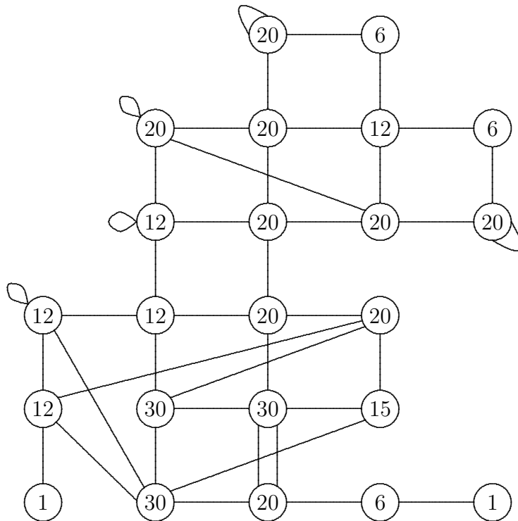
Figure 3: Representation B as a t -linkage of orbits of T = \langle a, b, c \rangle
