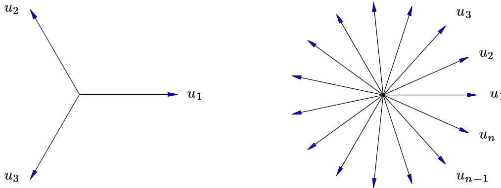
Fig. 1. Examples of n equally spaced vectors in \mathbb{R}^2 (which form a tight frame).
