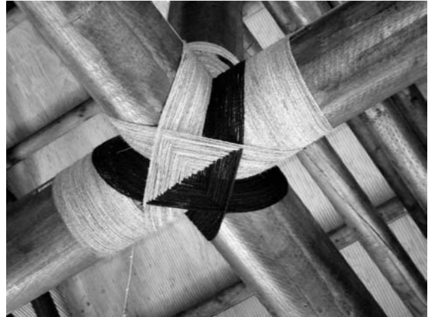
Figure 4: Lalava lashing.
