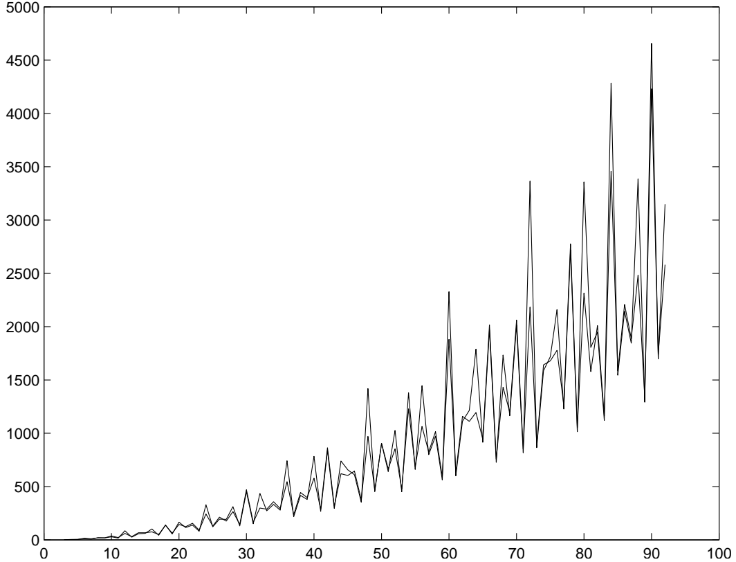
Figure 1: The number of harmonic frames of n distinct vectors for \mathbb{C}^3 (including noncyclic frames) as calculated by [WH06] together with a_{n,3} .
