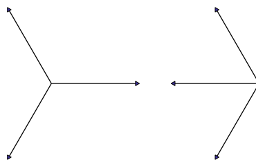
Fig. 1. The frames \Phi and \Phi' of Example 3, with |\text{Sym}(\Phi)| = 6 , |\text{Sym}(\Phi')| = 2 .
