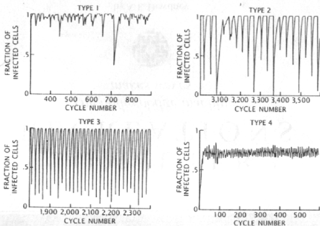
The four behaviors of the hodgepodge machine
