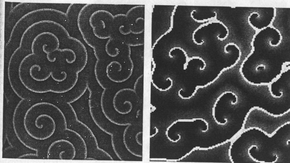
Wave phenomena in a Belousov-Zhabotinsky chemical reaction (left) and their hodgepodge counterparts (right)
