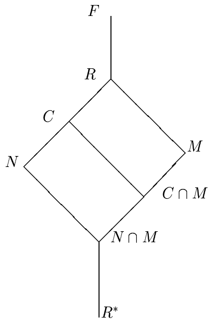
Figure 2: Case I - the characteristic subgroup contains the nucleus
