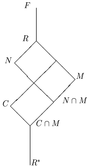
Figure 3: Case II - the characteristic subgroup is in the nucleus
