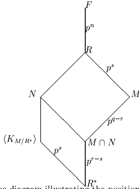
Figure 1: Lattice diagram illustrating the positions of various subgroups of F
